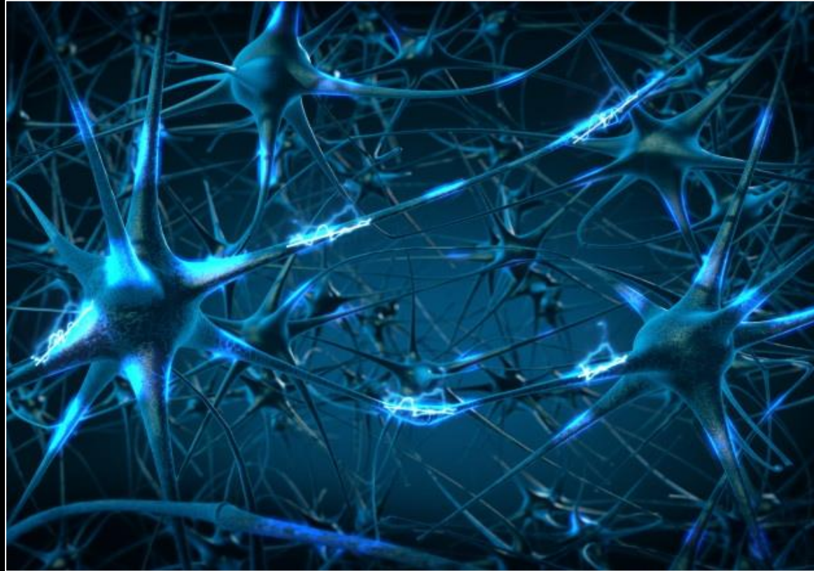
RED NEURONAL
